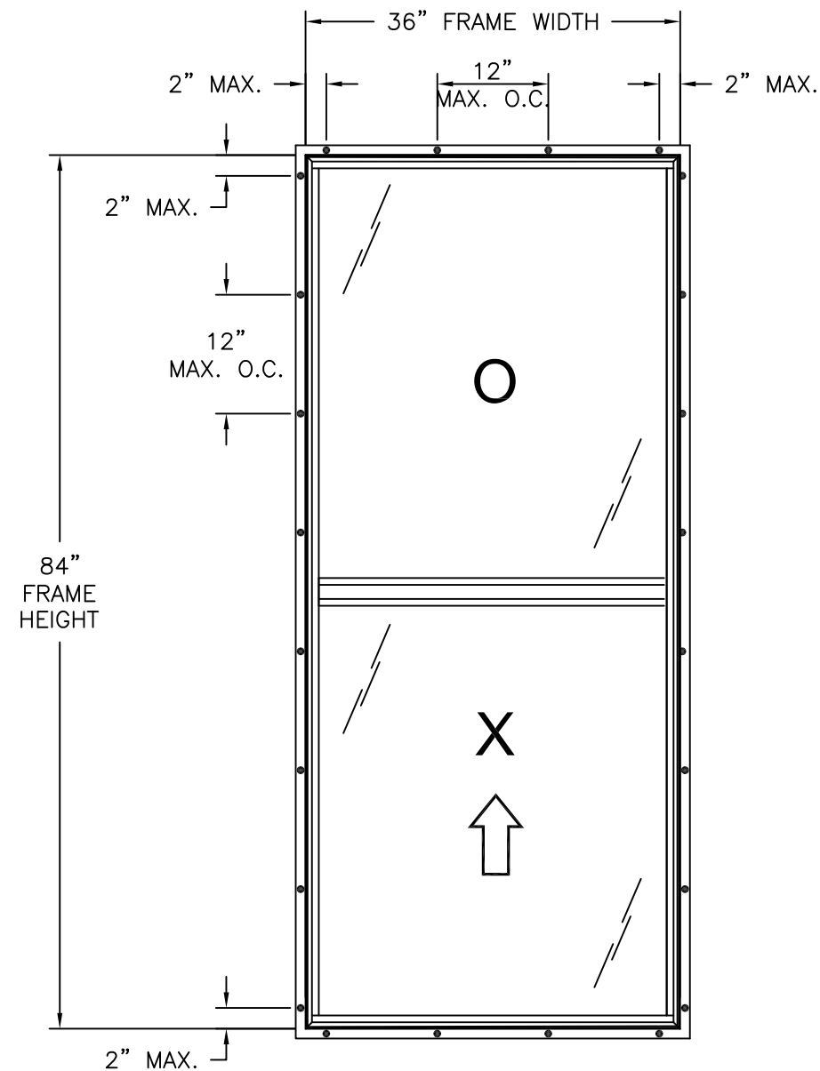
4000/4750 VINYL SINGLE HUNG WINDOW EXTERIOR VIEW
